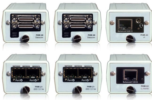
Hot swappable modules for Datacom, C37.94, Codirectional and VF.
