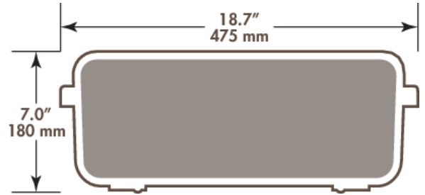
PiMPro Classic Case Width and Depth Dimensions
